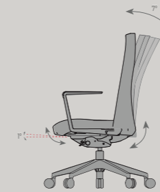
SYNCHRO MECHANISM TILT RATE Backrest tilt rate 7° to seat tilt rate 1° Auto-weight synchro control
