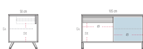
Block 20 - 2 section modules (1 door)
