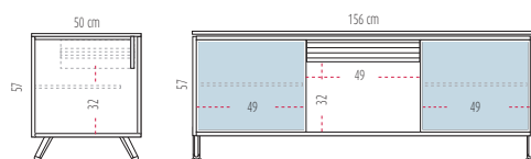
Block 20 - 3 section modules (2 doors)
